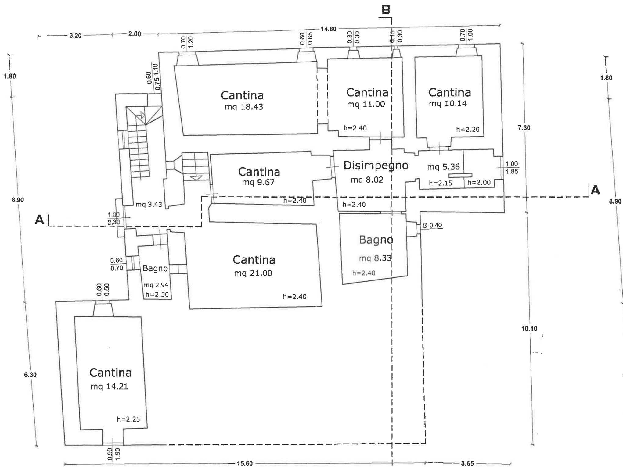
Piano Seminterrato 1
